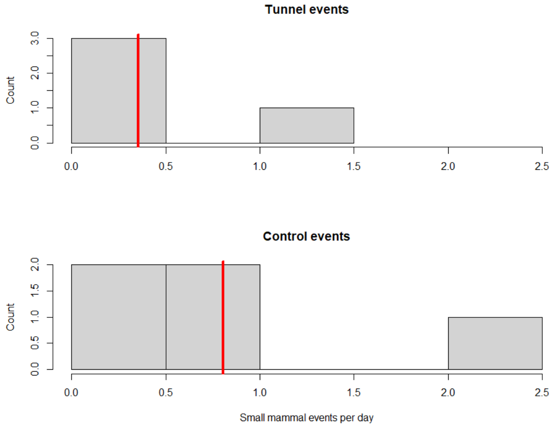
Figure 2. Counts of small mammal events detected at tunnel and control sites. Red lines depict mean events per day. An interval of 1 minute between detections of the same species was used to define events, and events were standardised to account for differences in camera functioning periods.
