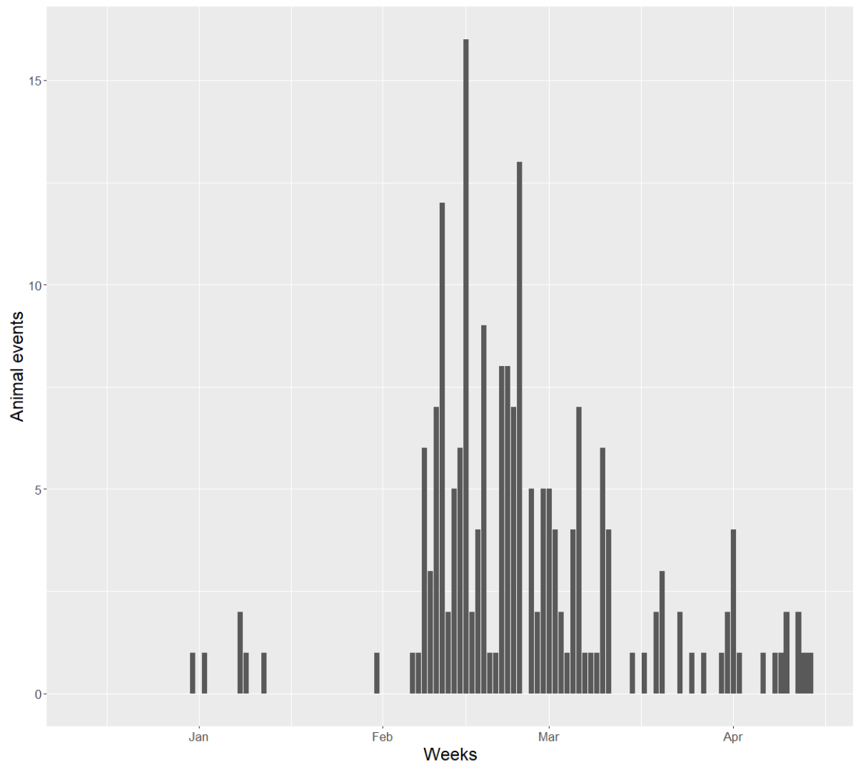
Figure 3. Animal events at tunnel sites for the first 6 months post-tunnel instillation (November 2020-April 2021). Animal activity is unstandardised as camera functioning was the same across all tunnel sites.
