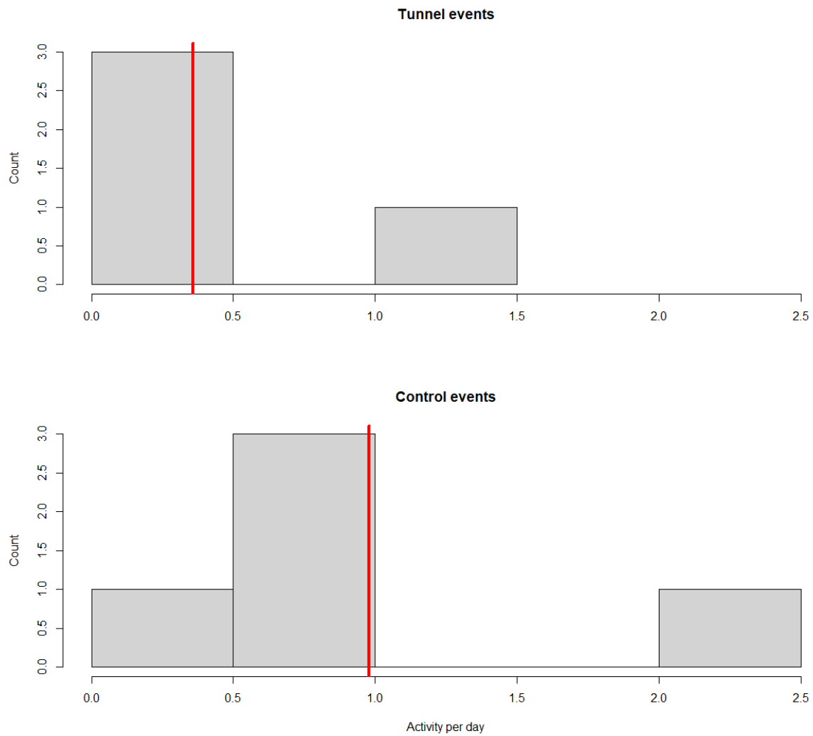
Figure 1. Counts of all animal events detected at tunnel and control sites. Red lines depict average number of events per day. An interval of 1 minute between detections of the same species was used to define events, and events were standardised to account for differences in camera functioning periods.
